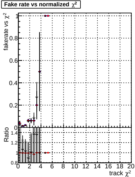
Fake rate vs. DOM mkFit baseline lowPT DOM mkFit baseline 6iter lowPT DOM mkFit TT Retrain v2 WP1 6iter ep3 lowPT
