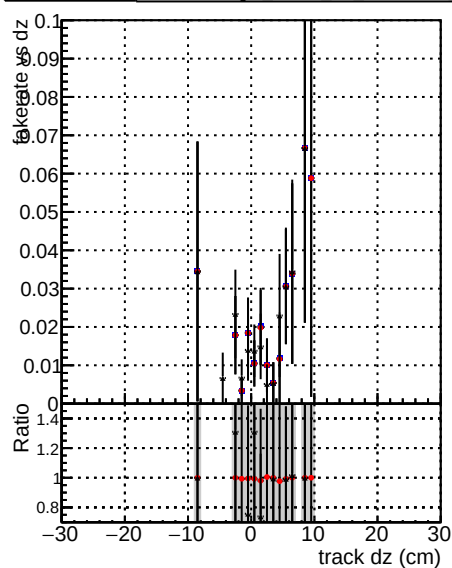
— DOM mkFit baseline lowPT — DOM mkFit baselineGiter lowPT — DOM mkFit TT RetrainV2 WP1 6iter ep3 lowPT
