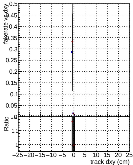
— DOM mkFit baseline lowPT — DOM mkFit baselineGiter lowPT — DOM mkFit TT RetrainV2 WP1 6iter ep3 lowPT
