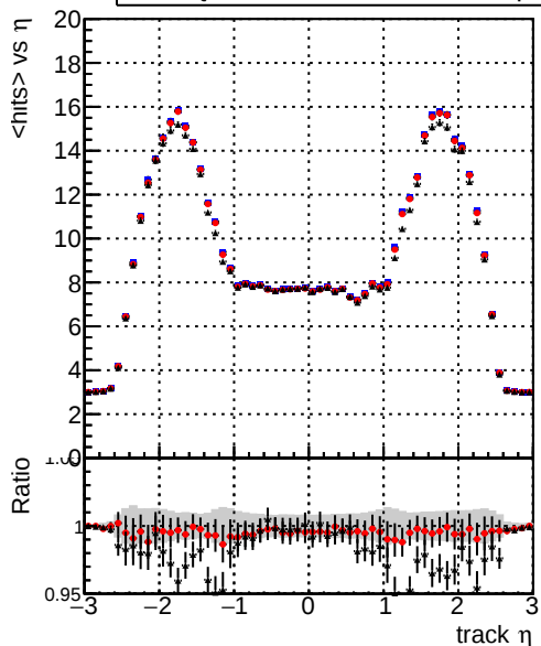
mean hits vs \eta — DQM_mkFit_baseline_lowPT — DQM_mkFit_baseline6iter_lowPT — DQM_mkFit_TT_RetrainV2_WP1_6iter_ep3_lowPT
