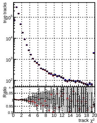
N of reco track vs. \chi^2 for DOM mkFit baseline_lowPT, DOM mkFit baseline_gitter_lowPT, and DOM mkFit V2_WP1_gitter_ep3_lowPT
