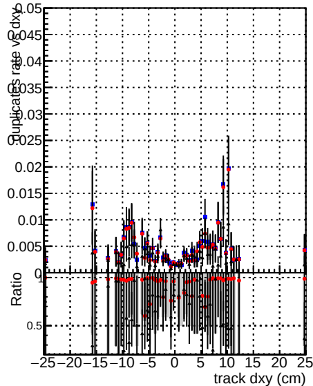
DOM mkFit baseline lowPT DOM mkFit baselineGiter lowPT DOM mkFit TT RetrainV2 WP1
