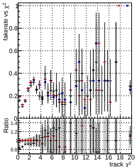
Fake rate vs. DOM mkFit baseline lowPT DOM mkFit baseline 6iter lowPT DOM mkFit 11 Retrain v2 WP1 6iter ep3 lowPT
