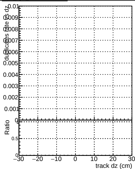
DOM mkFit baseline lowPT DOM mkFit baseline egger lowPT DOM mkFit TT RetrainV2 WP1 6iter ep3 lowPT
