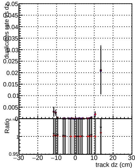
— DOM mkFit baseline lowPT — DOM mkFit baseline 6iter lowPT — DOM mkFit TT Retrain v2 WP1
