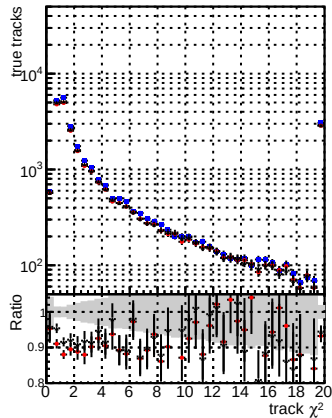
N of reco track vs. \chi^2 for various models: DOM mkFit baseline lowPT, DOM mkFit baseline gitter lowPT, DOM mkFit Retrain V2 WP1 gitter ep3 lowPT.
