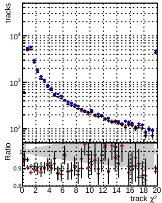
N of reco track vs. \chi^2 for various models: DOM mkFit baseline lowPT, DOM mkFit baseline gitter lowPT, DOM mkFit Retrain V2 WP1 gitter ep3 lowPT.
