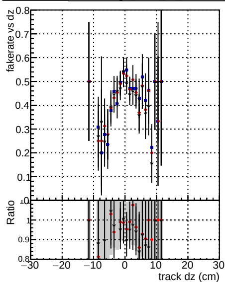
— DOM mkFit baseline lowPT — DOM mkFit baseline giter lowPT — DOM mkFit 1T Retrain2 WP1 6iter ep3 lowPT
