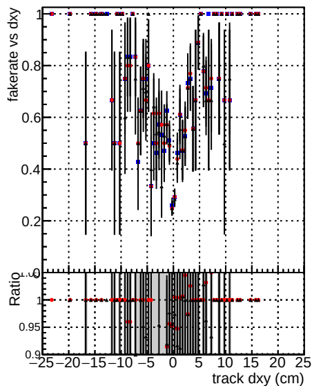
— DOM mkFit baseline lowPT — DOM mkFit baseline giter lowPT — DOM mkFit 1T Retrain2 WP1 6iter ep3 lowPT
