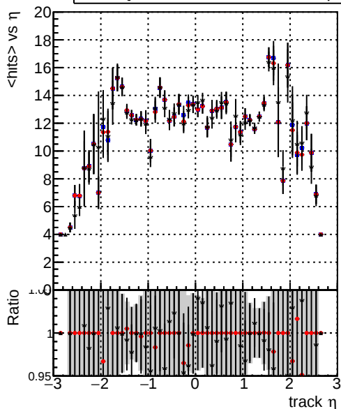
mean hits vs \eta — DQM_mkFit_baseline_lowPT — DQM_mkFit_baseline6iter_lowPT — DQM_mkFit_TT_RetrainV2_WP1_6iter_ep3_lowPT
