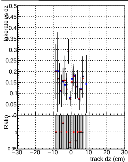
Fake rate vs dz Legend: DOM mkFit baseline lowPT DOM mkFit baseline Gitter lowPT DOM mkFit TT Retrain v2 WP1 Gitter ep3 lowPT
