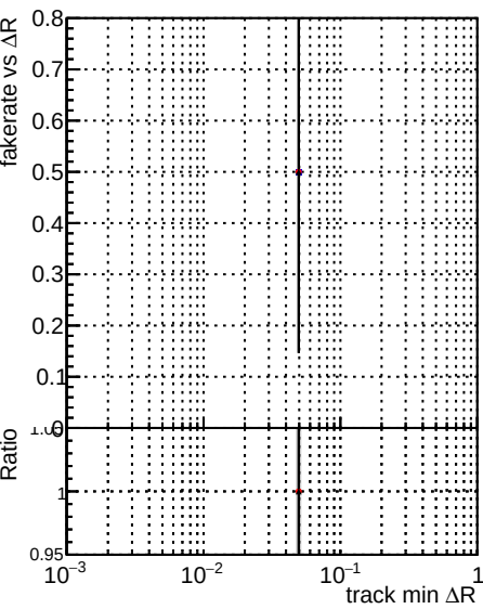
Legend: - \Delta R mkFit baseline_lowPT - \Delta R mkFit baseline6iter_lowPT - \Delta R mkFit TT_RetrainV2_WP1_6iter_ep3_lowPT
