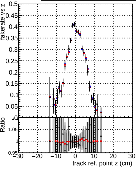
DOM_mkFit_baseline_lowPT DOM_mkFit_baseline6iter_lowPT DOM_mkFit_TT_RetrainV2_WP1_6iter_ep3_lowPT
