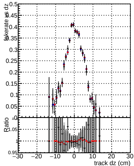
—•— DOM mkFit baseline lowPT —•— DOM mkFit baseline gite lowPT —•— DOM mkFit TT Retrain v2 WP1 6iter ep3 lowPT
