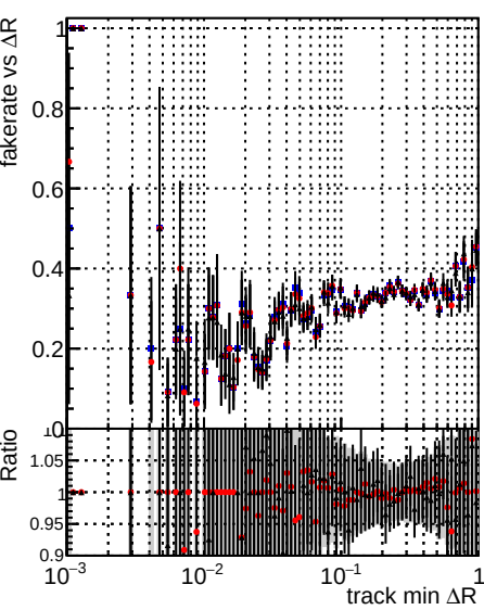
Legend: DQM_mkFit_baseline_lowPT (black), DQM_mkFit_baseline6iter_lowPT (red), DQM_mkFit_TT_RetrainV2_WP1_6iter_ep3_lowPT (blue)
