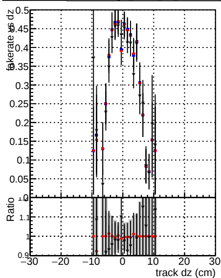
Fake rate vs dz Legend: DOM mkFit baseline lowPT DOM mkFit baseline giter lowPT DOM mkFit TT Retrain2 WP1 giter ep3 lowPT
