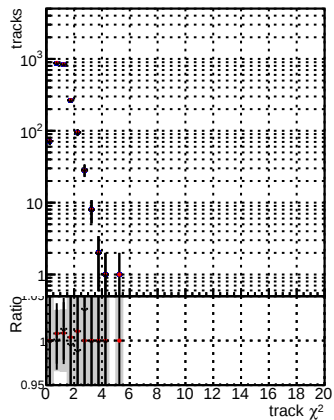
N of reco track vs. \chi^2 for various models: DOM mkFit baseline lowPT (blue), DOM mkFit baseline giter lowPT (red), DOM mkFit Retrain V2 WP1 6iter ep3 lowPT (black).
