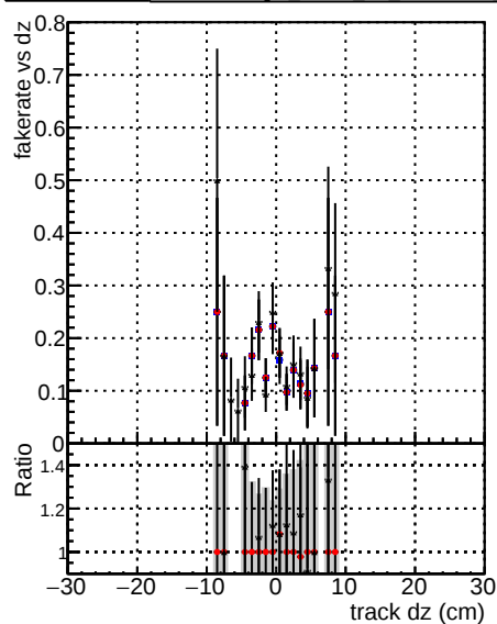
Fake rate vs dz DOM mkFit baseline lowPT DOM mkFit baseline giter lowPT DOM mkFit TT Retrain2 WP1 giter ep3 lowPT
