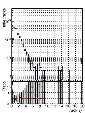
N of reco track vs. \chi^2 DGM mkFit baseline lowPT DGM mkFit baseline 6iter lowPT DGM mkFit Retrain V2 WP1 6iter ep3 lowPT
