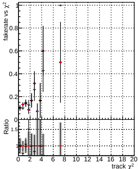
Fake rate vs. — DOM mkFit baseline_lowPT — DOM mkFit baseline_6iter_lowPT — DOM mkFit TT RetrainV2 WP1 6iter ep3_lowPT
