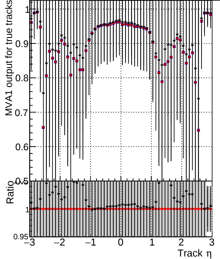
MVA1 of associated tracks (recoToSim) vs. track \eta Legend: DQM_mkFit_baseline_lowPT (blue squares) DQM_mkFit_baseline6iter_lowPT (red circles) DQM_mkFit_TT_RetrainV2_WP1_6iter_ep3_lowPT (black stars)
