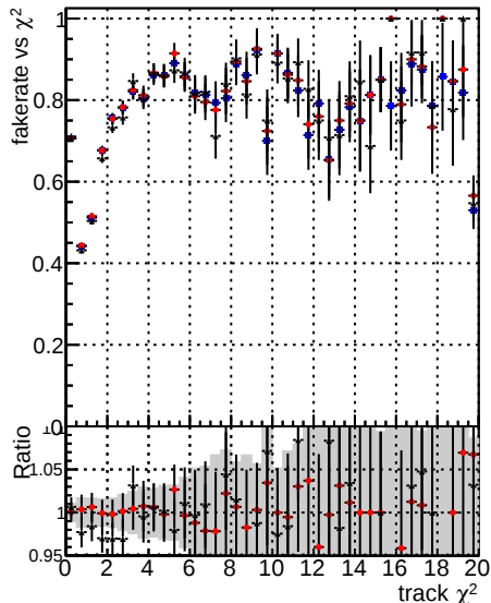
Fake rate vs. \chi^2 Legend: DOM mkFit baseline lowPT (blue stars) DOM mkFit baseline 6iter lowPT (red stars) DOM mkFit 11 Retrain v2 WP1 6iter ep3 lowPT (black stars)
