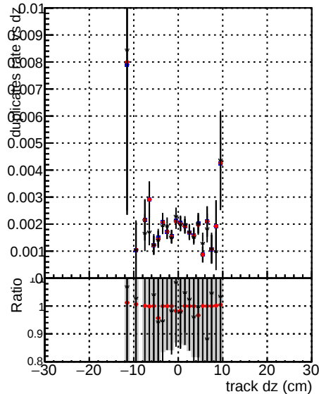
— DOM mkFit baseline_lowPT — DOM mkFit baseline_lowPT — DOM mkFit TT_Retrain_v2_lowPT
