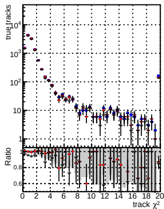
N of reco track vs. \chi^2 for baseline_lowPT, baseline_6iter_lowPT, baseline_6iter_ep3_lowPT, RetrainV2_WP1_6iter_ep3_lowPT
