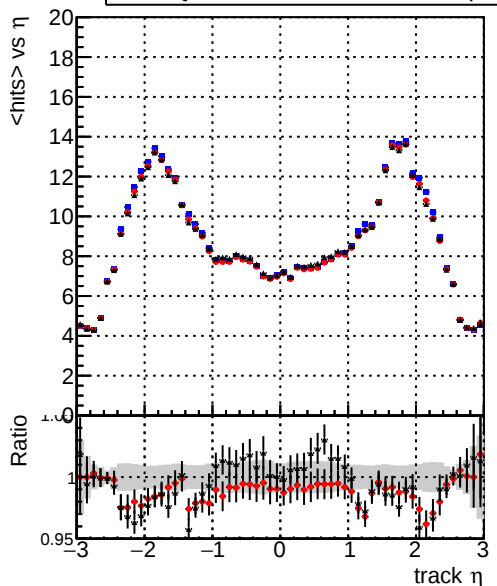
mean hits vs \eta — DQM_mkFit_baseline_lowPT — DQM_mkFit_baseline6iter_lowPT — DQM_mkFit_TT_RetrainV2_WP1_6iter_ep3_lowPT
