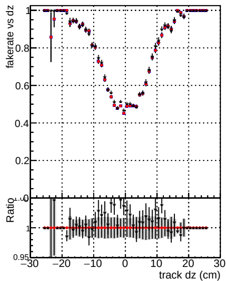
DOM mkFit baseline DOM mkFit baseline6iter DOM mkFit RetrainV2 WP2 6iter ep3
