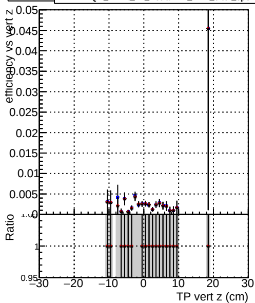
Efficiency —●— DQM_mkFit_baseline6iter —▲— DQM_mkFit_TT_RetrainV2_WP2_6iter_ep3
