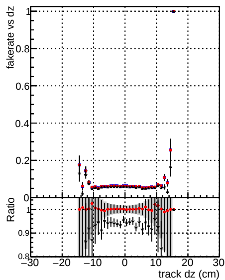
Fake rate vs dz DOM mkFit baseline DOM mkFit baseline6iter DOM mkFit 11 RetrainV2 WP2 6iter ep3
