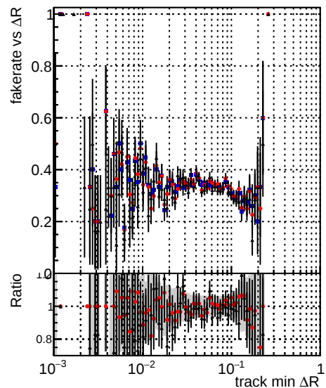
Fake rate vs \Delta R(\text{track, jet}) Legend: DQM_mkFit_baseline (black line with dots) DQM_mkFit_baseline6iter (red line with dots) DQM_mkFit_TT_RetrainV2_WP2_6iter_ep3 (blue line with dots)
