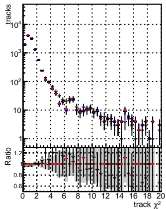
N of reco track vs. \chi^2 for DGM mkFit baseline, DGM mkFit baseline gitter, and DGM mkFit V2 Retrain
