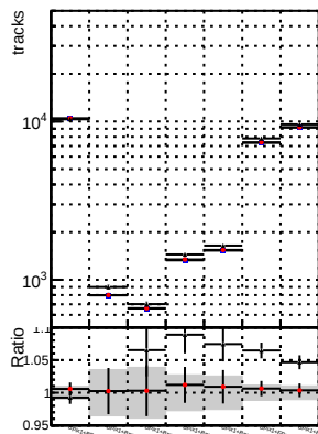
N of reco track vs. \chi^2 DOM mkFit baseline DOM mkFit baseline6iter DOM mkFit V1 Retrain V2 WP2 6iter ep3
