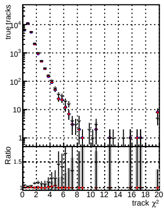
N of reco track vs. \chi^2 DOM mkFit baseline DOM mkFit baseline6iter DOM mkFit V1 Retrain V2 WP2 6iter ep3
