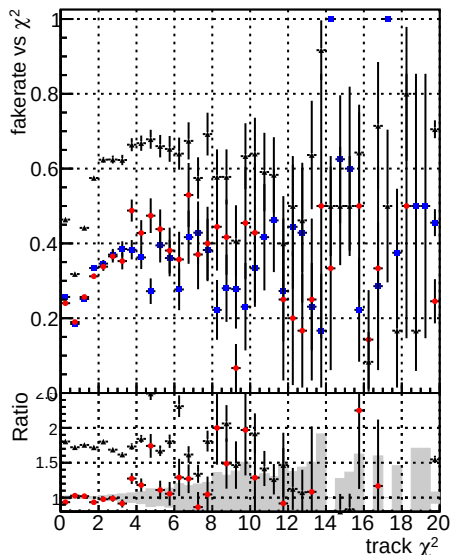
Fake rate vs. DOM mkFit baseline DOM mkFit baselineGitter DOM mkFit 11 RetrainV2 WP2 6iter ep3
