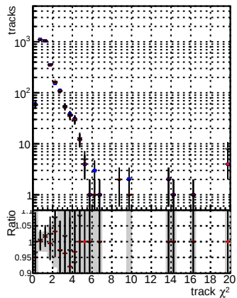
N of reco track vs. \chi^2 DOM mkFit baseline DOM mkFit 6iter DOM mkFit 11 RetrainV2 WP2 6iter ep3
