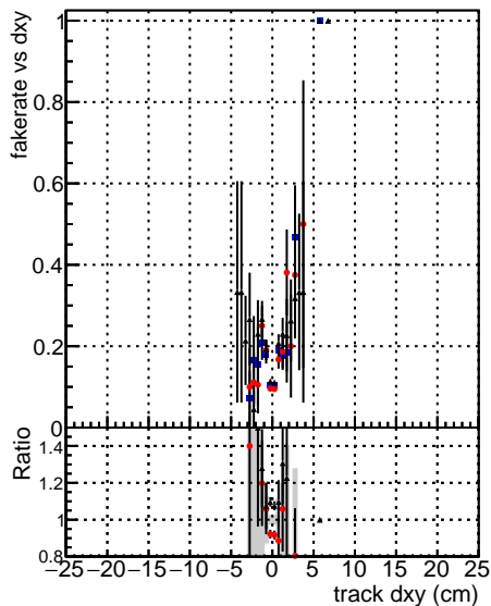
■ DGM mkFit baseline ● DGM mkFit baseline 6iter ▲ DGM mkFit 11 Retrain V2 WP2 6iter ep3
