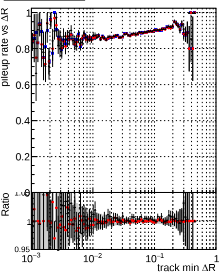
Legend: DQM_mkFit_baseline (black line with error bars), DQM_mkFit_baseline6iter (red line with error bars), DQM_mkFit_TT_RetrainV2_WP2_6iter_ep3 (black line with error bars)
