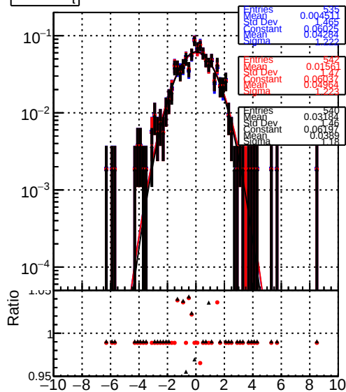
BDM mkt RetrainV2 RetrainV2 WP2 6iter_ep3
