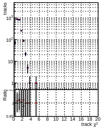
N of reco track vs. \chi^2 for DQM mkFit baseline, DQM mkFit baseline gitter, and DQM mkFit RetrainV2 WP2 6iter ep3
