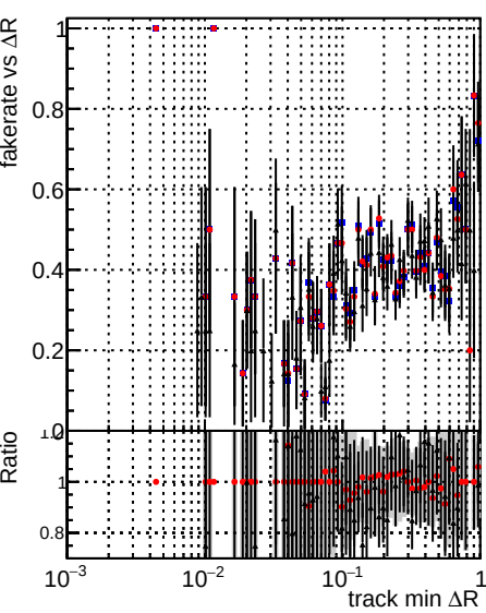
Fake rate vs \Delta R (track, jet) DQM_mkFit_baseline DQM_mkFit_baseline6iter DQM_mkFit_TT_RetrainV2_WP2_6iter_ep3
