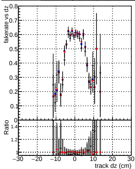
Fake rate vs dz Legend: DOM mkFit baseline (black line), DOM mkFit baselineGitter (red line), DOM mkFit 11 RetrainV2 WP2 6iter ep3 (blue line)
