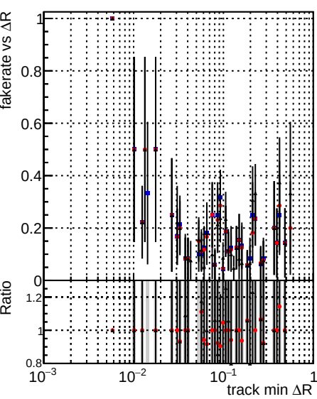
Legend: DQM_mkFit_baseline (black), DQM_mkFit_baseline6iter (red), DQM_mkFit_TT_RetrainV2_WP2_6iter_ep3 (blue)
