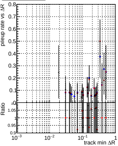
Legend: DQM_mkFit_baseline (black), DQM_mkFit_baseline6iter (red), DQM_mkFit_TT_RetrainV2_WP2_6iter_ep3 (blue)
