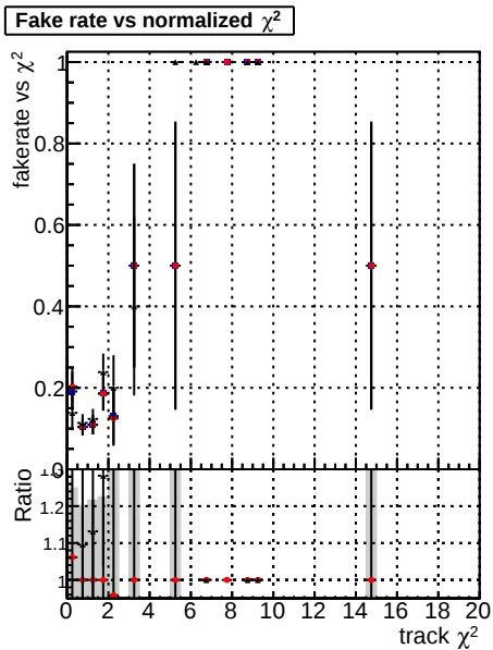
Fake rate vs. Legend: DOM mkFit baseline (black line) DOM mkFit baseline6iter (red line) DOM mkFit RetrainV2 WP2 6iter ep3 (blue line)
