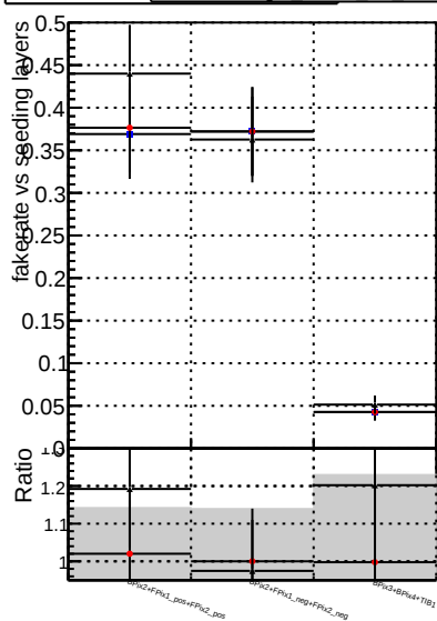
Fake rate vs. Legend: DOM mkFit baseline (black line) DOM mkFit baseline6iter (red line) DOM mkFit RetrainV2 WP2 6iter ep3 (blue line)
