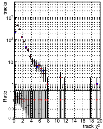
N of reco track vs. \chi^2 DGM mkFit baseline DGM mkFit baseline+6iter DGM mkFit V2 Retrain
