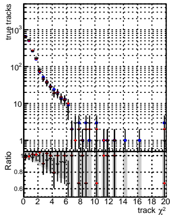
N of reco track vs. \chi^2 for DGM mFit baseline WP2 6iter ep3
