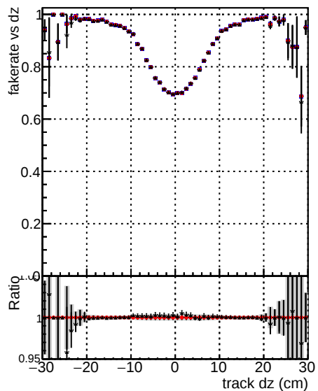
— DOM mkFit baseline — DOM mkFit baseline6iter — DOM mkFit 11 RetrainV2
