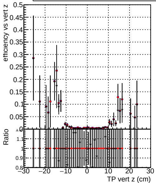
Efficiency vs. TP vert z (cm) Legend: - DQM_mkFit_baseline (blue line with dots) - DQM_mkFit_baseline6iter (red line with dots) - DQM_mkFit_TT_RetrainV2_WP2_6iter_ep3 (black line with dots)
