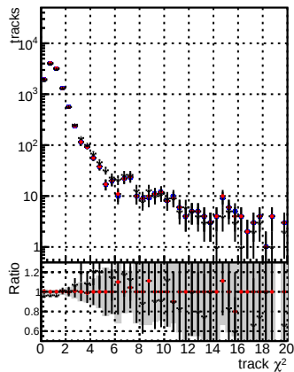
N of reco track vs. \chi^2 DGM mkFit baseline DGM mkFit baseline gitter DGM mkFit V2 Retrain WP2 6iter ep3
