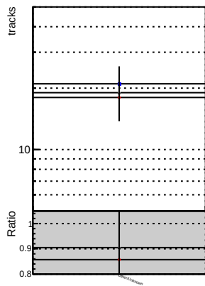
N of reco track vs. \chi^2 for various models
