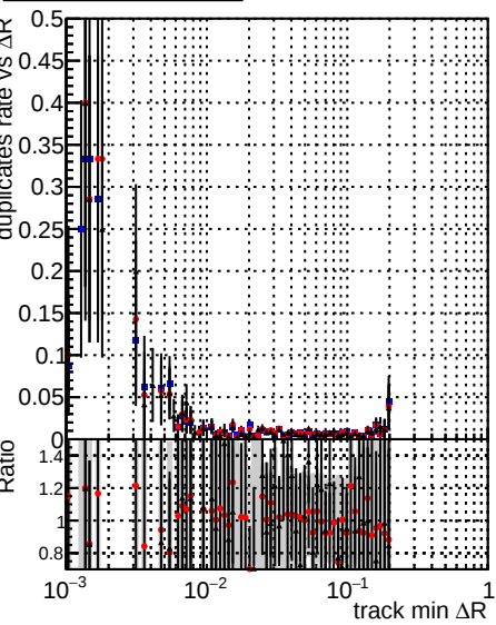
Legend: DQM_mkFit_baseline (black), DQM_mkFit_baseline6iter (red), DQM_mkFit_TT_RetrainV2_WP2_6iter_ep3 (grey)
