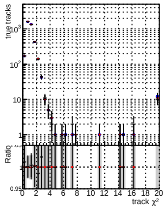
N of reco track vs. \chi^2 for baseline, 6iter, and WP2 6iter ep3 models.
